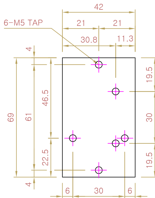
BRACKET - ②
