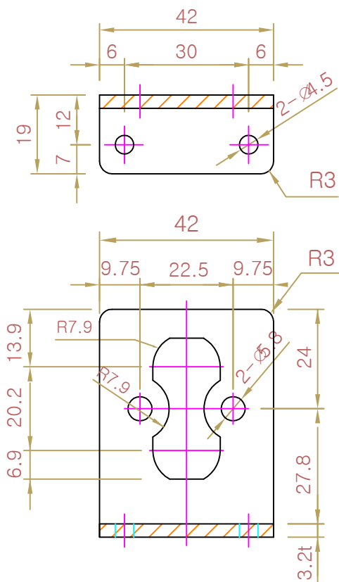
BRACKET - ①
