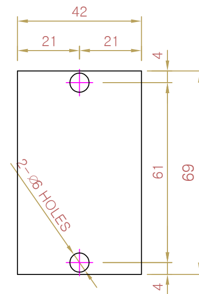
BRACKET - ③
